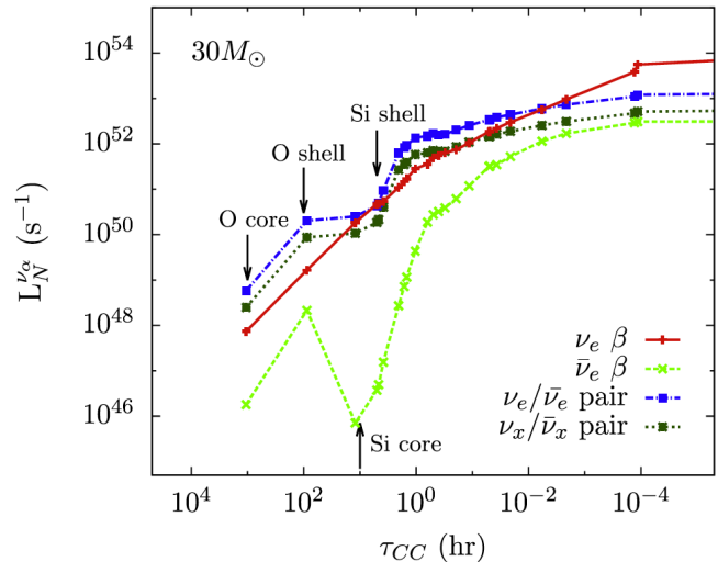
Figure 1. Neutrino luminosities leading up to core collapse. A few hours before collapse, the luminosity of beta-process neutrinos outshines that of any other neutrino flavor or origin. Credit: Patton et al. 2017
