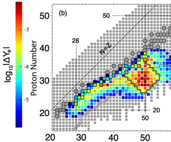
Figure 1. Nuclear chart indicating the contribution of specific isotopes to the change in electron fraction during the late stage of core-collapse supernovae. Nuclei near N=50 , above ^{78}\text{Ni} are particularly important.
